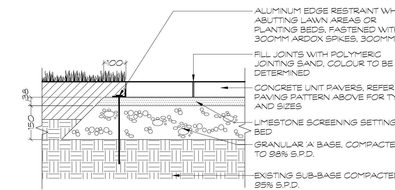
D5 CONCRETE UNIT PAVER DETAIL 1:10
