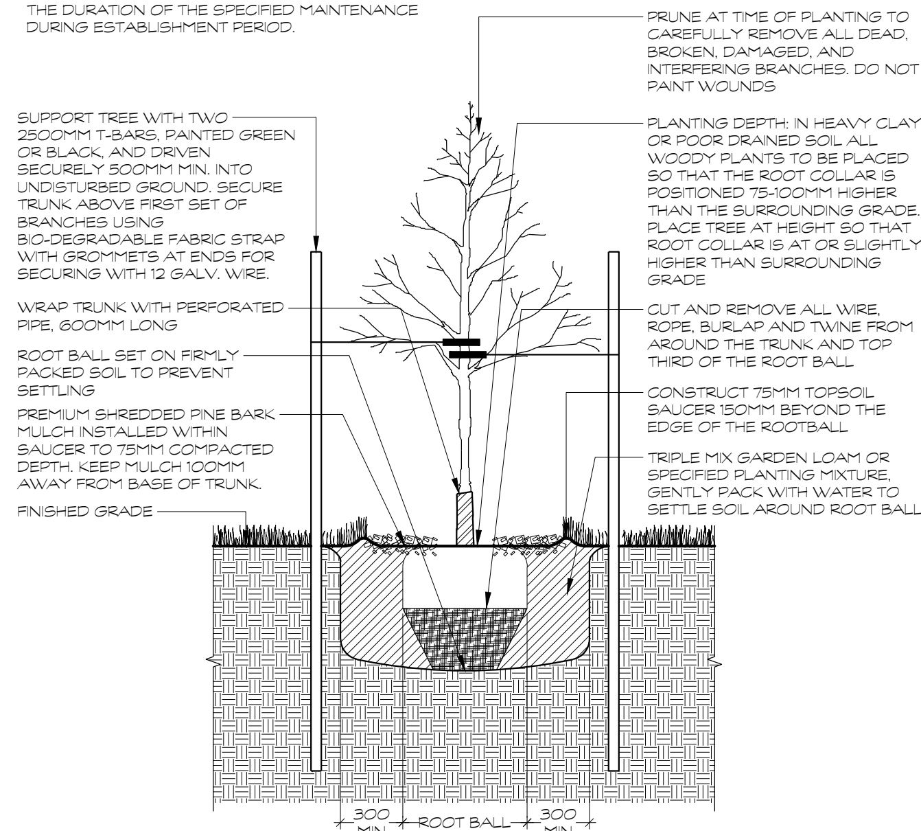
D1 DECIDUOUS TREE PLANTING 1:25
