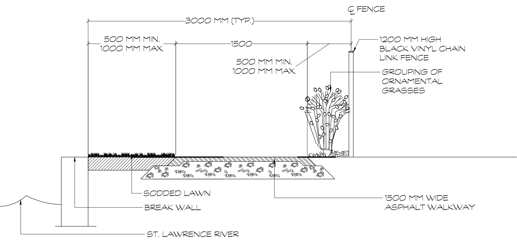
D6 TYPICAL SECTION THRU ASPHALT WALKWAY 1:25
