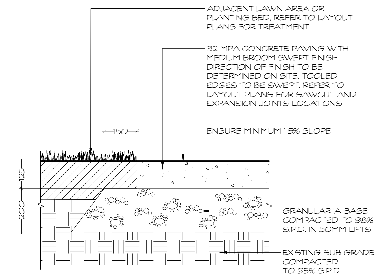
D4 CONCRETE PAVING 1:10
