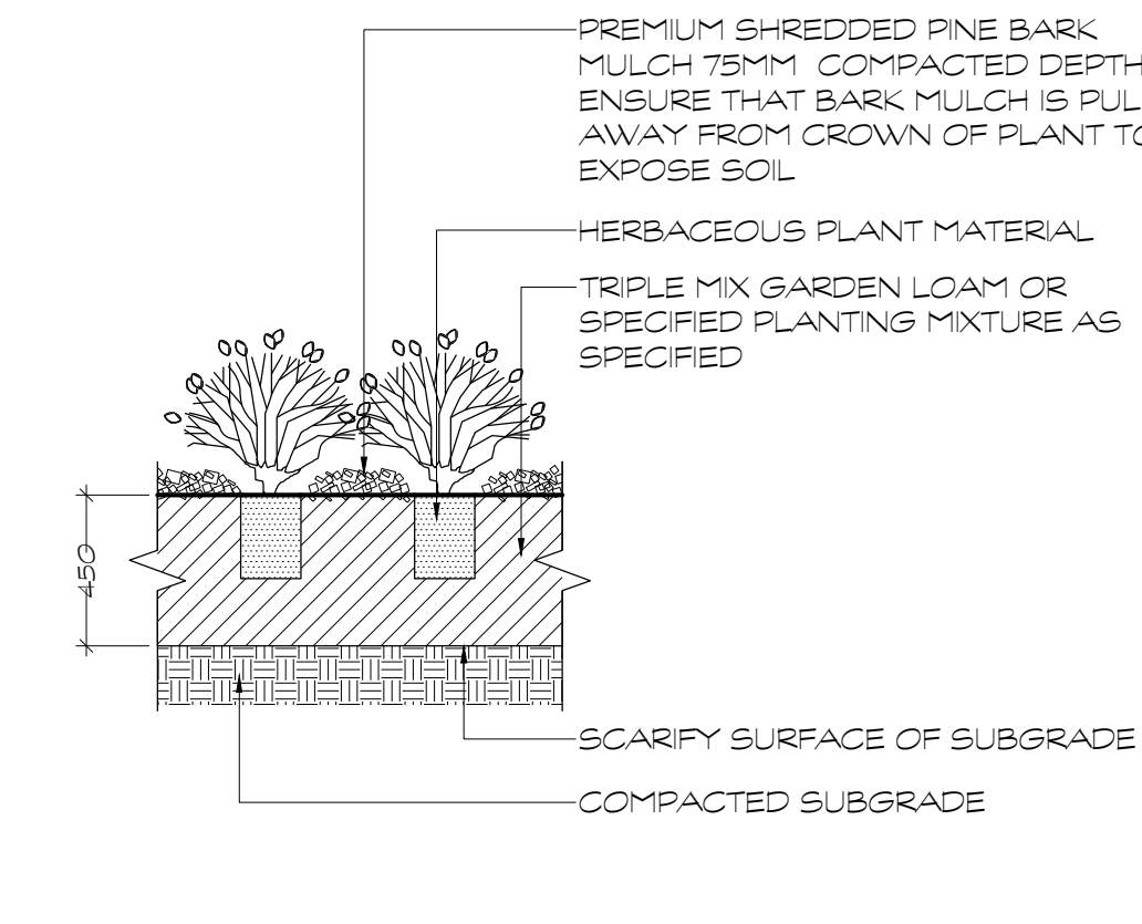
D3 HERBACEOUS PLANTING 1:25
